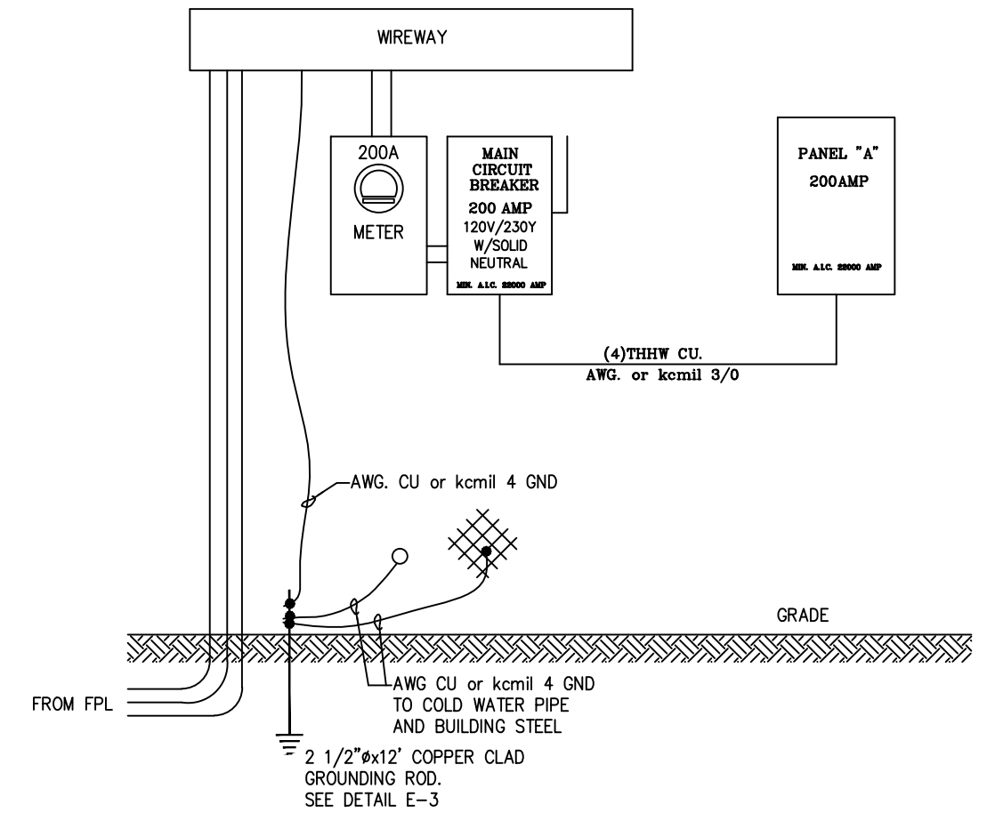
ELECTRICAL RISER
