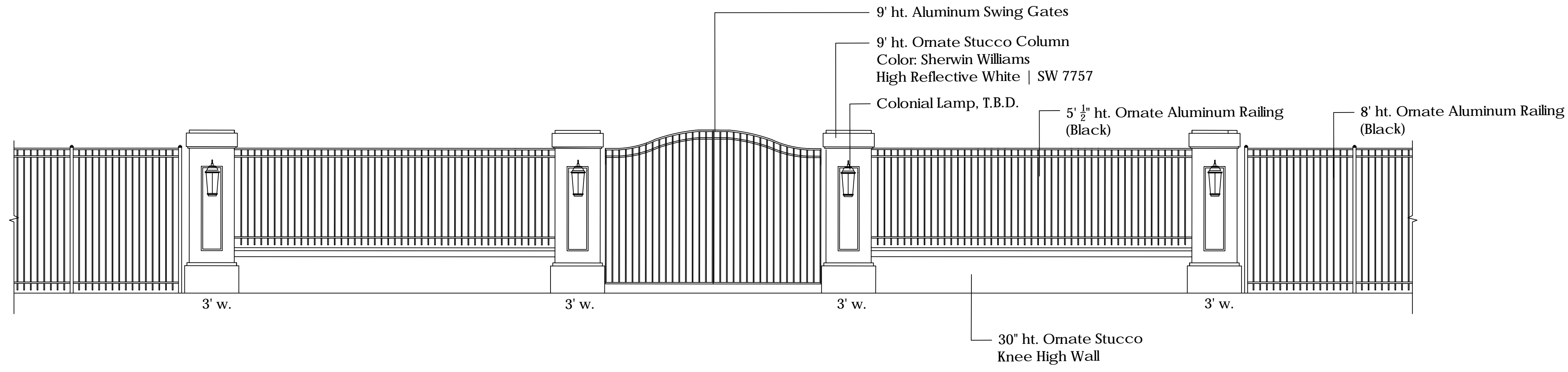
TYPICAL ENTRY GATE AND RAILING DETAIL N.T.S.
